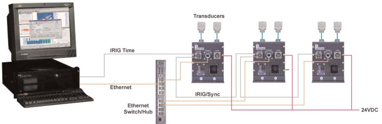
Typical 7220 Installation
